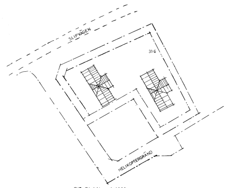
SIT PLAN 1:1000
