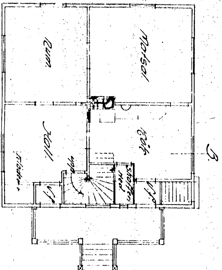
Bottenplan 8
