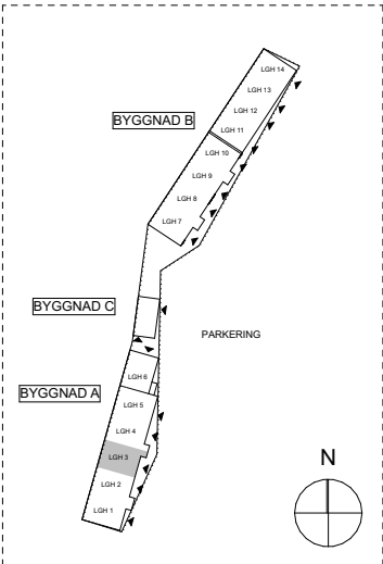
SITUATIONSPLAN
