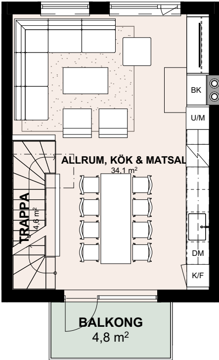
PLAN 2
